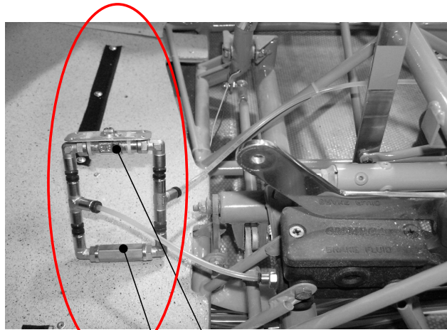
Park-brake-shutoff-valve
